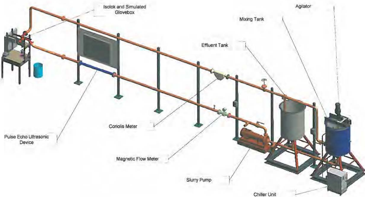
Figure 2-3. Schematic of Remote Sampler Demonstration Test Platform
