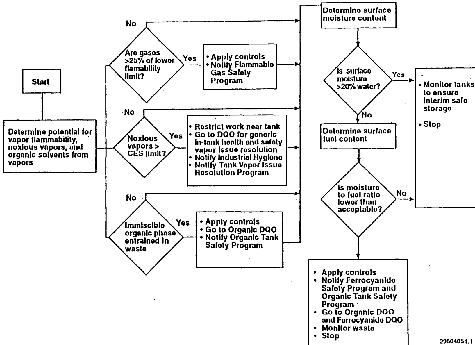
Figure 1-1. Logic Diagram for Safety Screening DQO Process.
