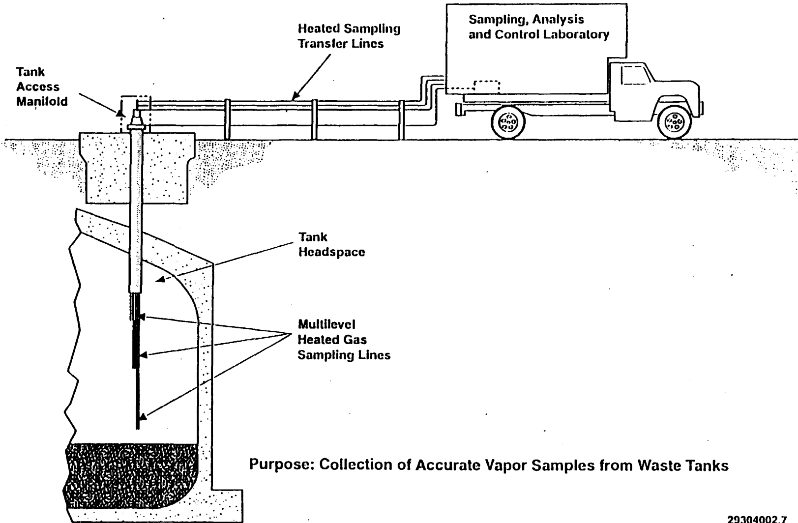
Figure 7-1. Vapor Sampling System
