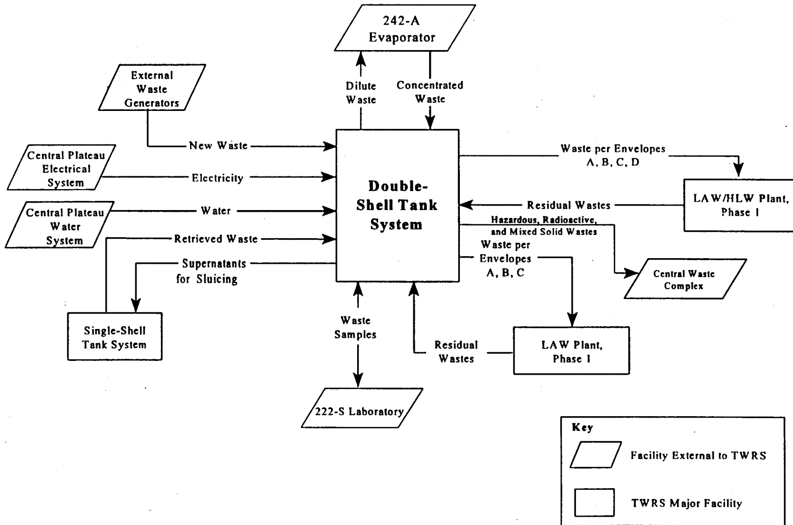
Figure 3-3. Double-Shell Tank System Interface Diagram.
