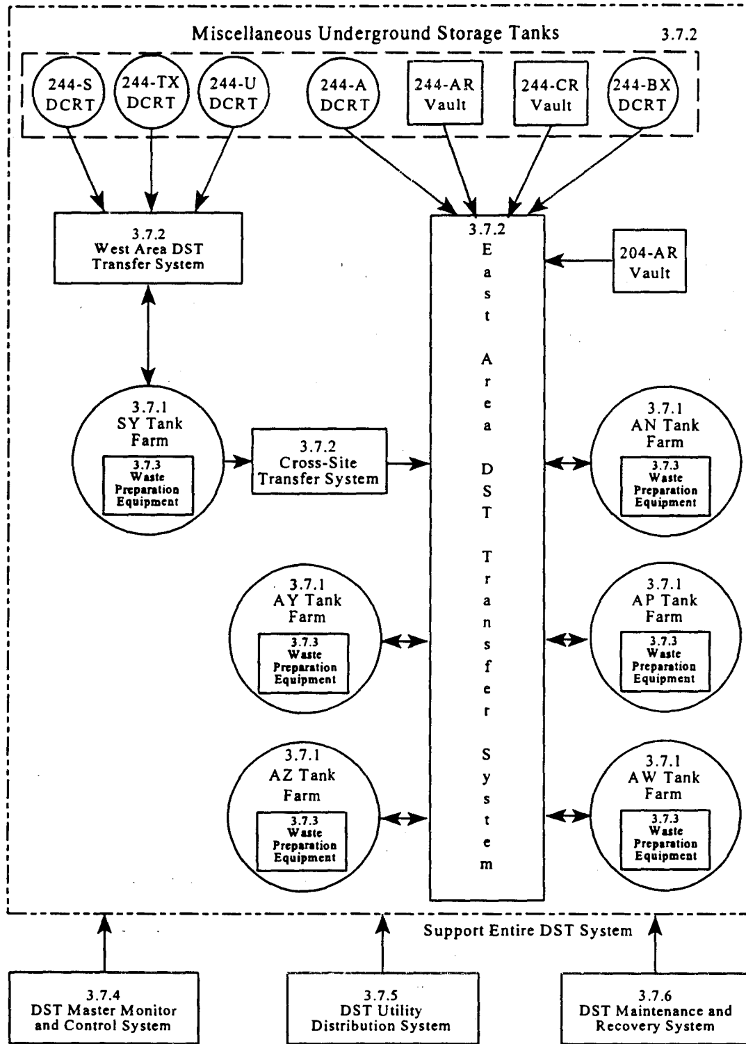
Figure 3-4. Phase 1 Double-Shell Tank System.
