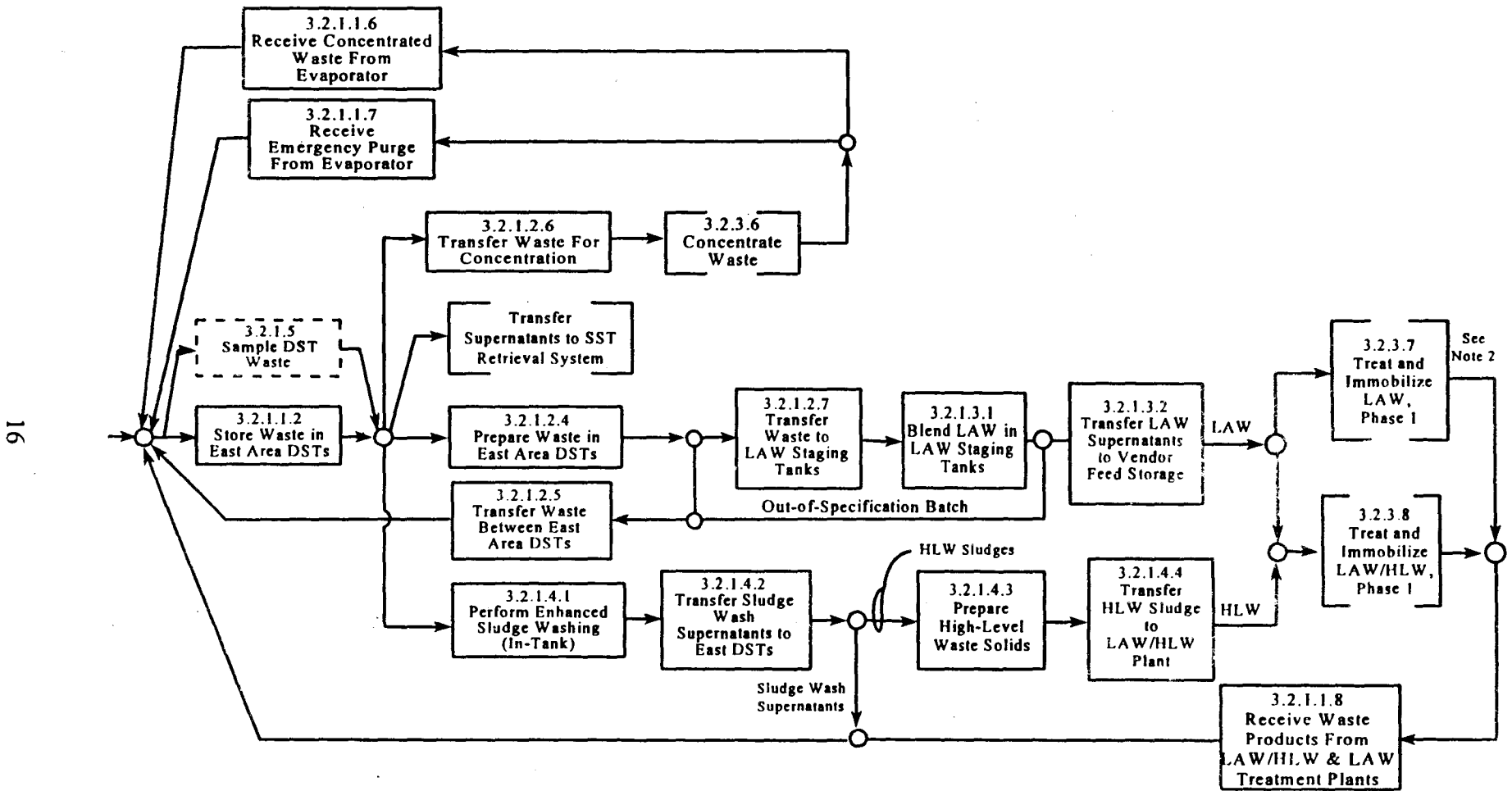
Figure 3-2. Double-Shell Tank System Functional Flow Block Diagram (Sheet 2 of 3).
