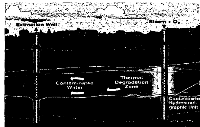
Hydrous Pyrolysis/Oxidation
